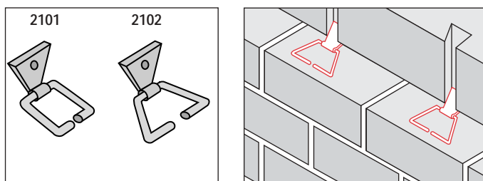
Dovetail with Triangular or Rectangular Tie
